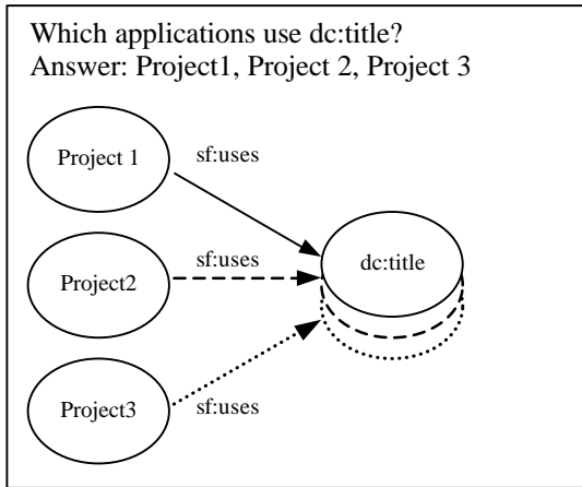
Figure 8. Joining statements as a basis for queries
