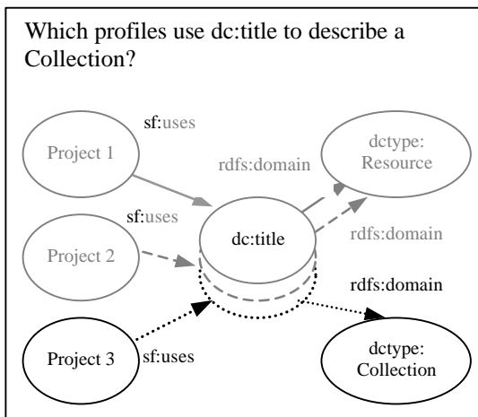
Figure 9. Narrowing a search
