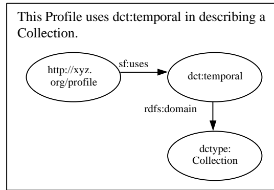
Figure 2. Specify a class of object to which it refers
