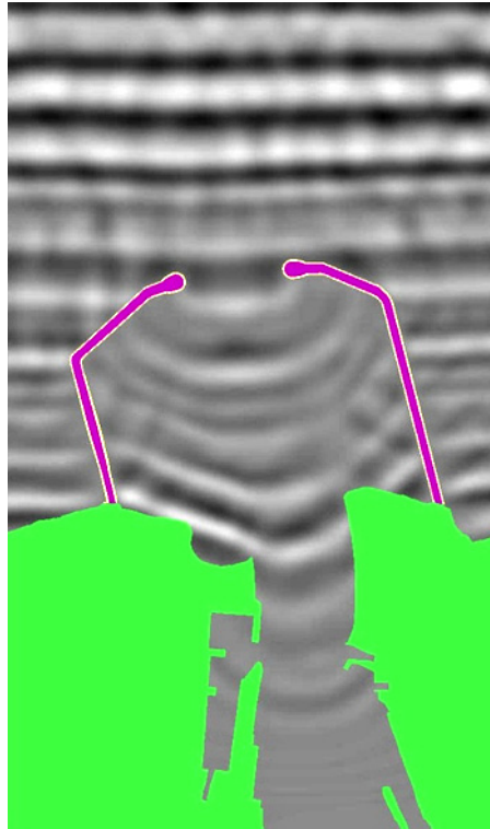
Figure 8. Instantaneous surface elevations in MILDwave of waves propagating and penetrating the harbour, for the final configuration of the new breakwaters.
