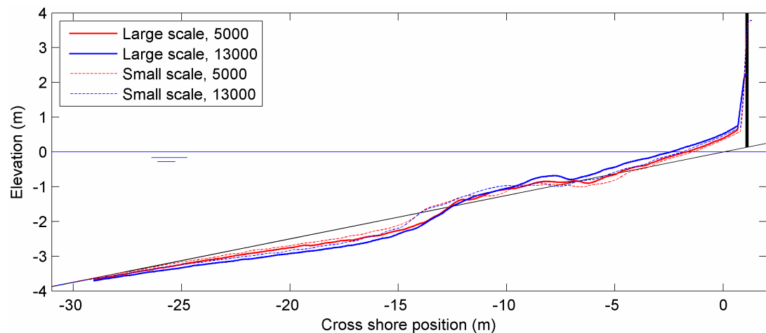
Figure 21. Comparison between large-scale and small-scale tests with seawall.
