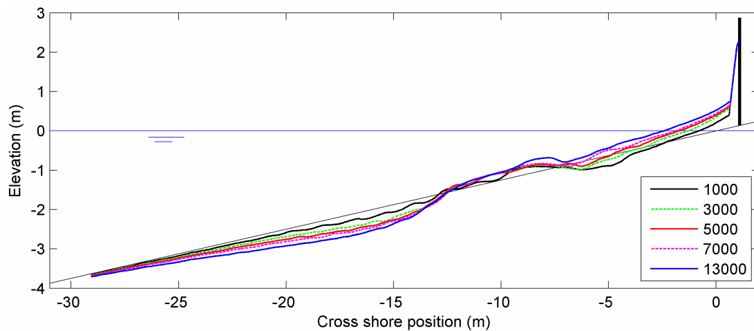
Figure 20. Large-scale tests: Development in time of gravel beach with seawall.
