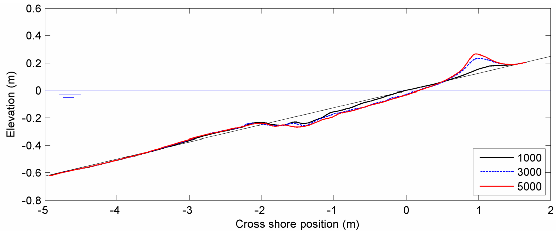
Figure 6. Small-scale tests: Development in time (with sand in pores).
