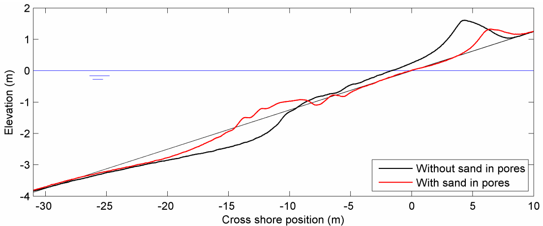
Figure 17. Large-scale tests: Comparison of profiles with and without sand in pores.
